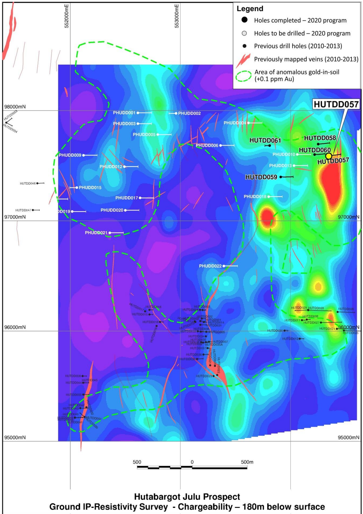
Figure 6: Hutabargot Julu Prospect Drill Hole Locations on IP Chargeability (2012 Ground IP-Resistivity Survey) Note: Red-yellow indicate high chargeability, blue-magenta indicate low chargeability
