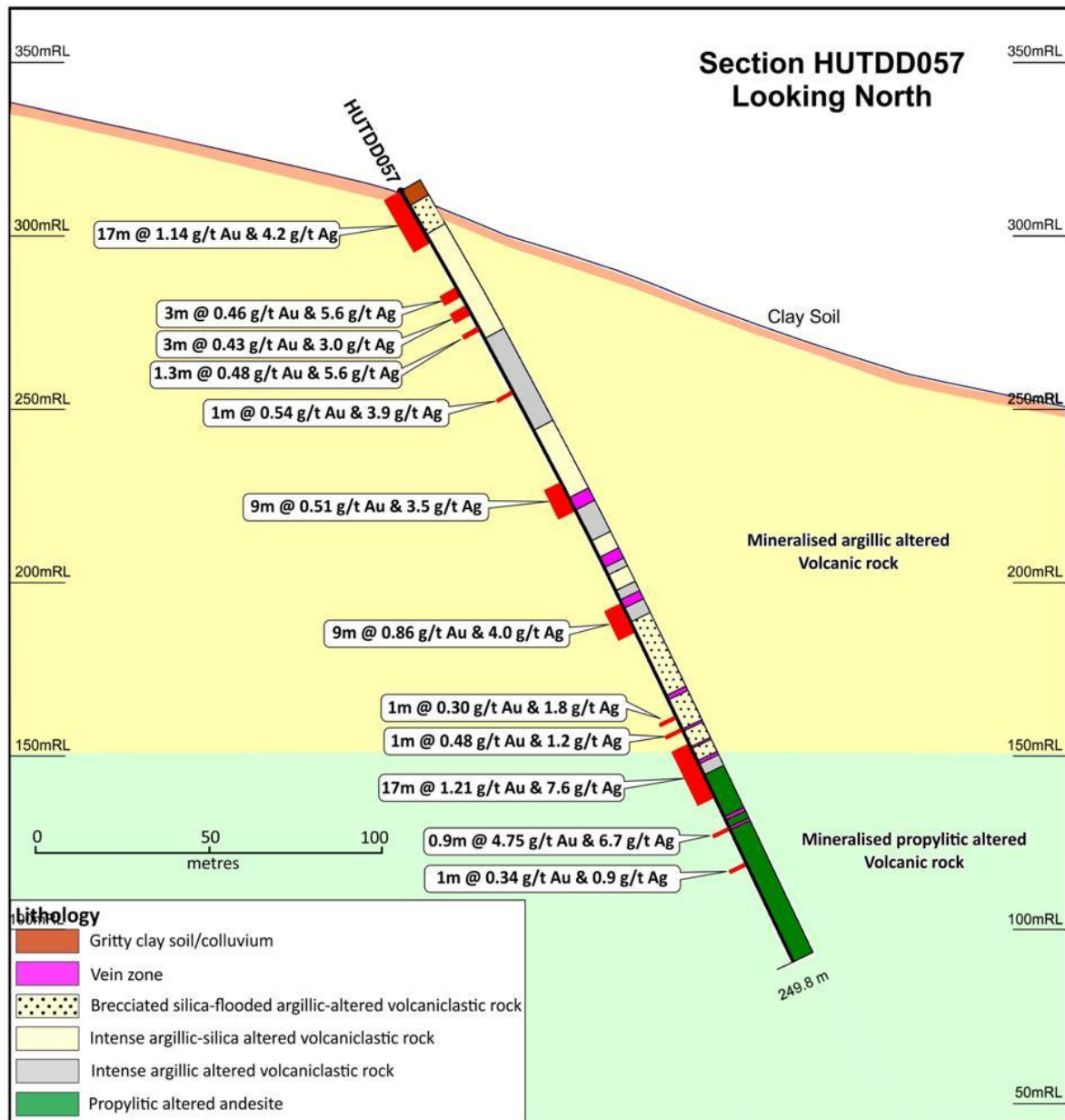
Figure 1: Hutabargot Julu Prospect Section 97,600 N – Drill hole HUTDD057 – Lithology & Au-Ag Results
