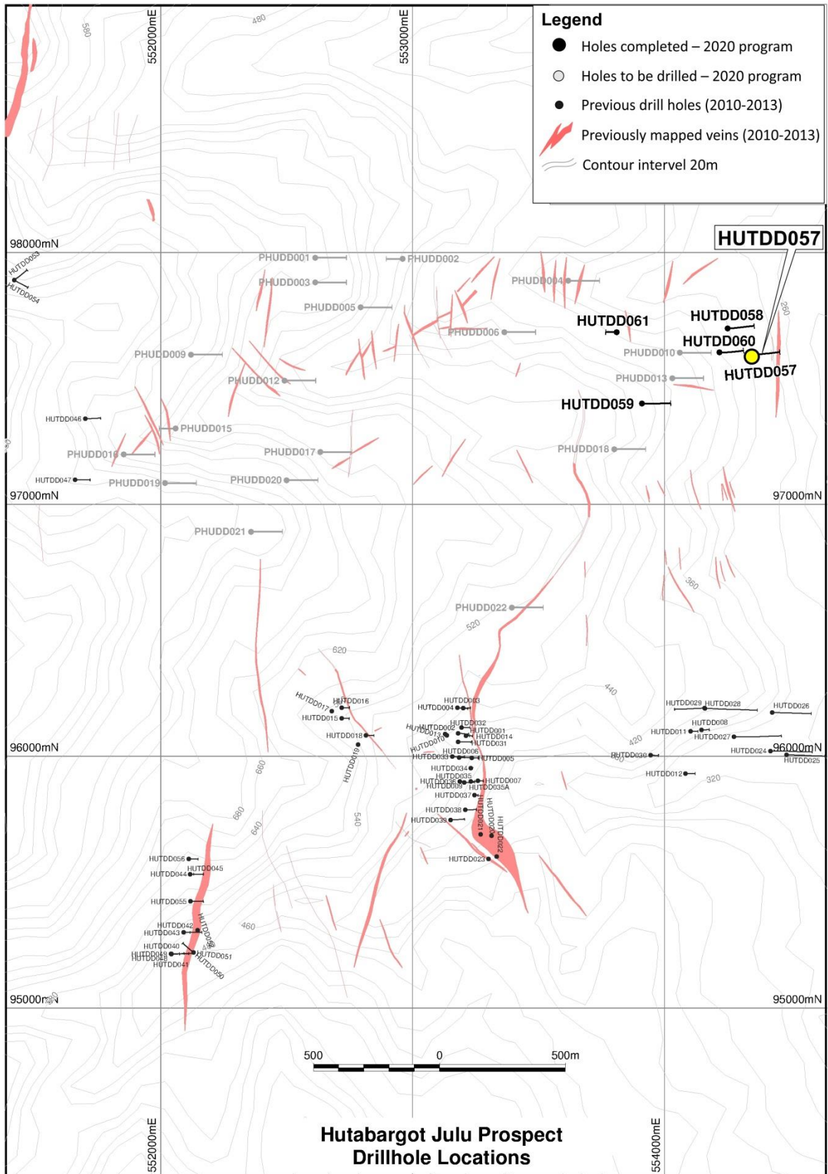
Figure 3: Hutabargot Julu Prospect – Drill Hole Location Plan highlighting HUTDD057
