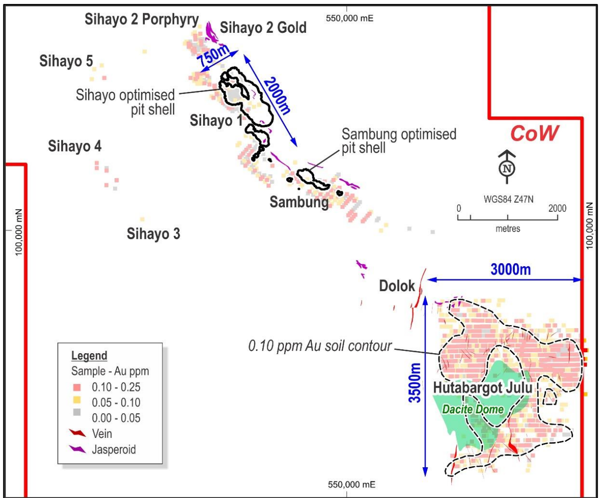
Figure 2: Hutabargot Julu Prospect Location Extensive Gold-Soil Anomaly within the Sihayo Gold Belt
