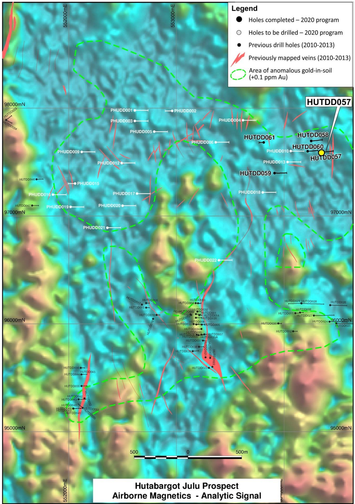
Figure 5: Hutabargot Julu Prospect Drill Hole Locations on TMI-Analytic Signal Magnetics (2012 Airborne Survey) (Reprocessed by Intrepid Geophysics)
