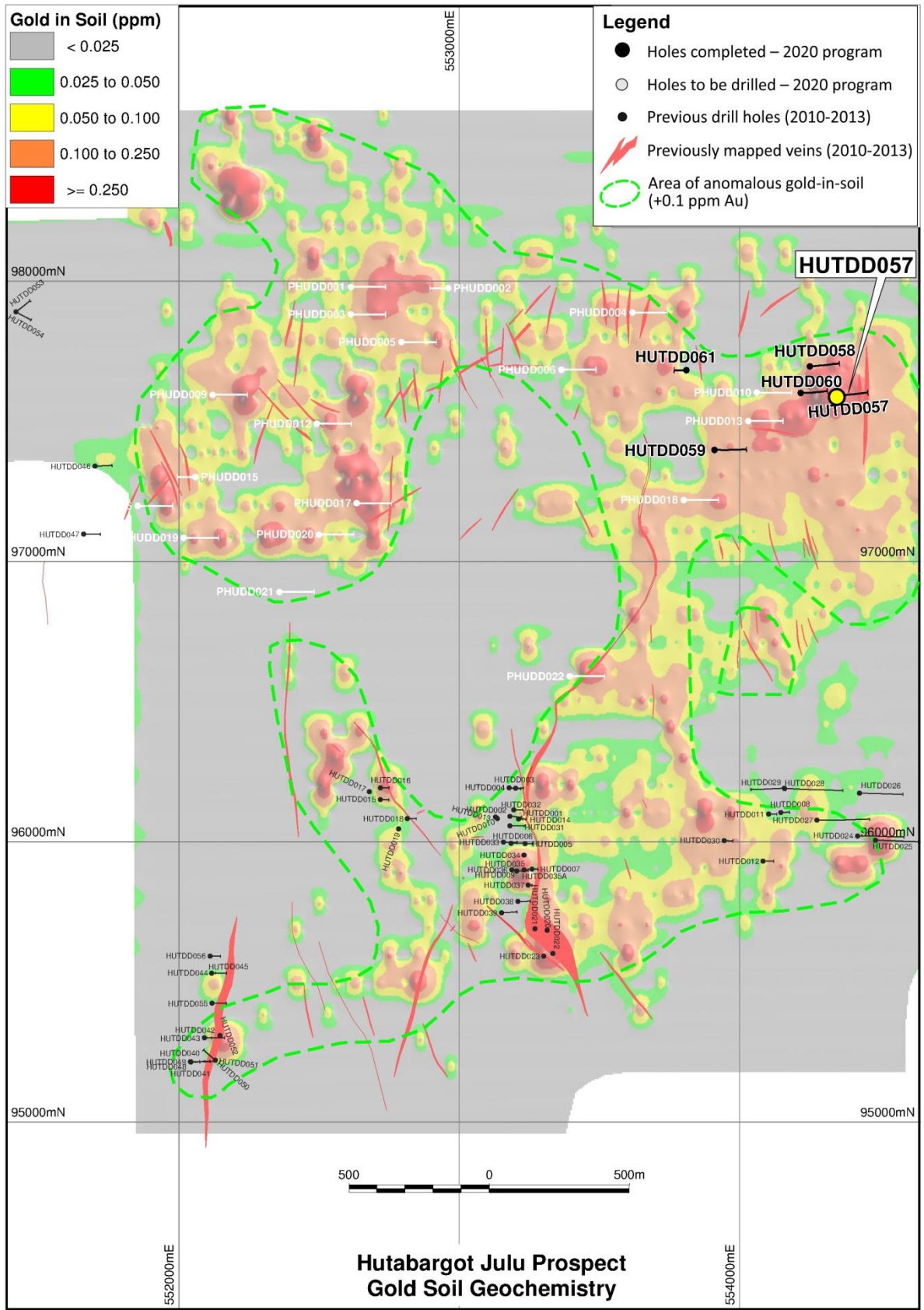
Figure 4: Hutabargot Julu Prospect Drill Hole Locations on Gold Soil Geochemistry (2012 Soil Survey)
