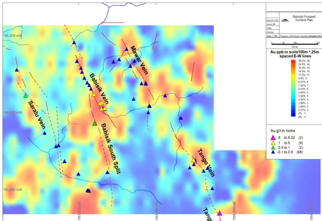
Figure 12: Babisik Prospect Surface Plan
