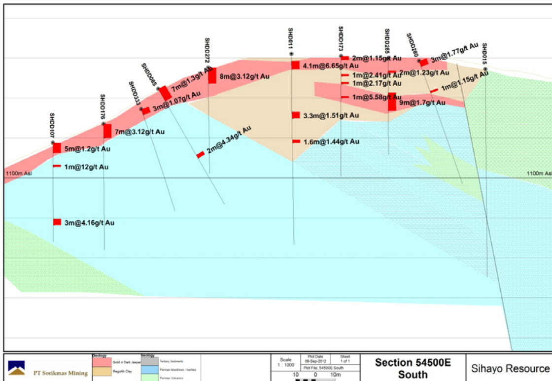
Figure 8: Cross Section Enlargement 54500E shows Significant Gold Intercepts. Located on Figure 7 & 3
