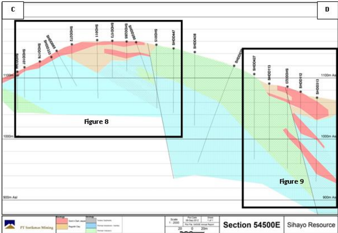
Figure 7: Geology Cross Section 54500E of Sihayo Resource looking NW. Located on Figure 3
