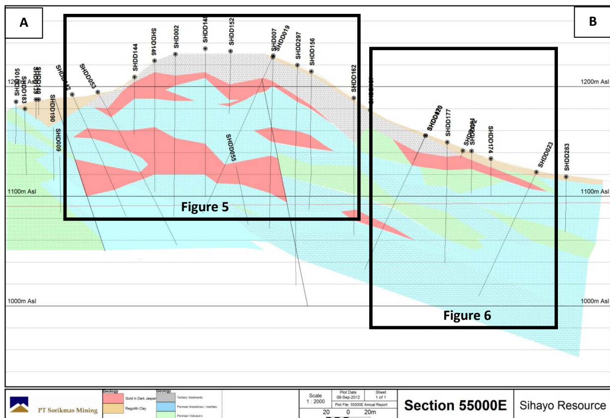
Figure 4: Geology Cross Section 55000E of Sihayo Resource looking NW. Located on Figure 3
