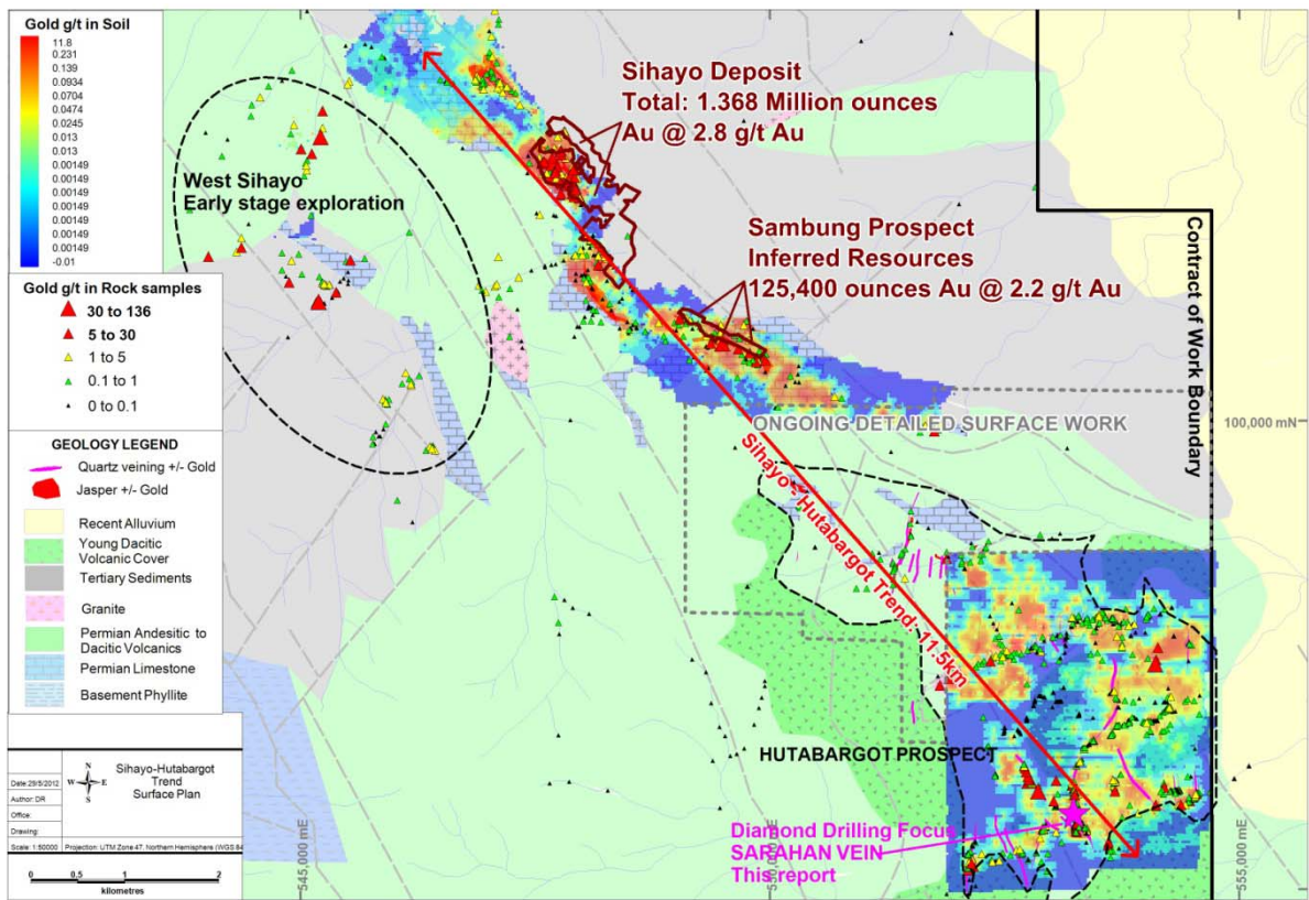
Figure 10: Sihayo Pungkut – Hutabargot Julu Trend
