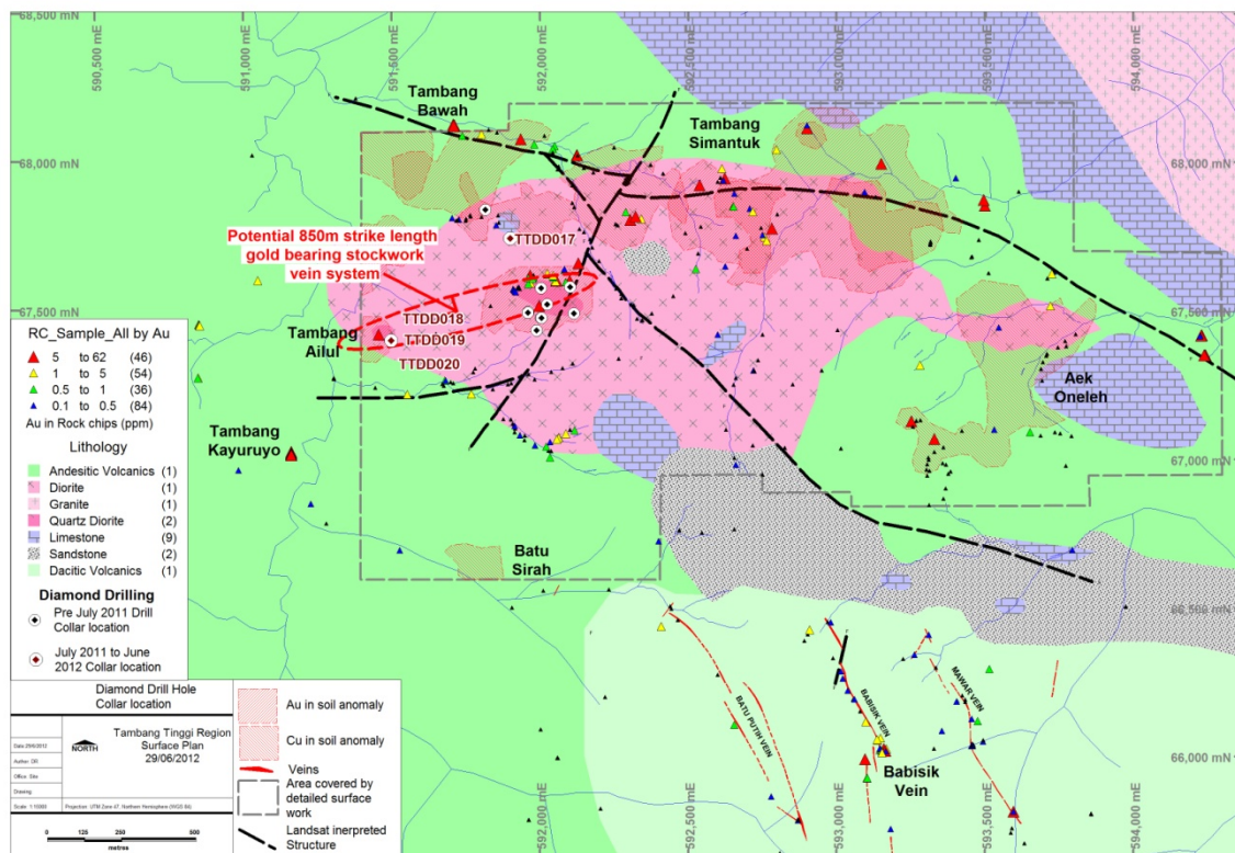
Figure 13: Tambang Tinggi Surface Plan
