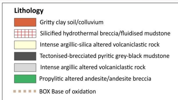
Figure 4. Section of HUTDD063 & HUTDD065 (looking North)
