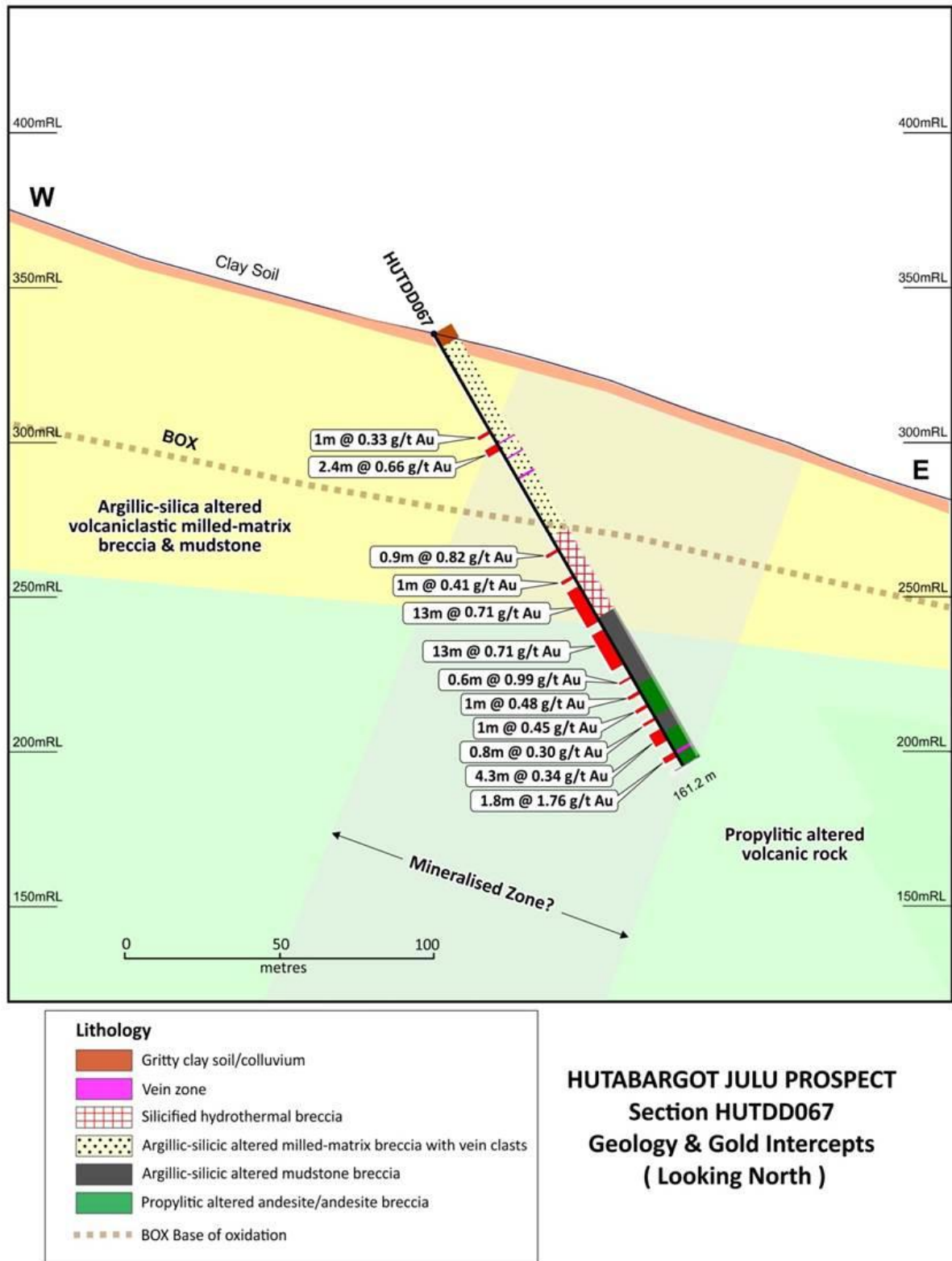
Figure 5. Section of HUTDD067 (looking North)
