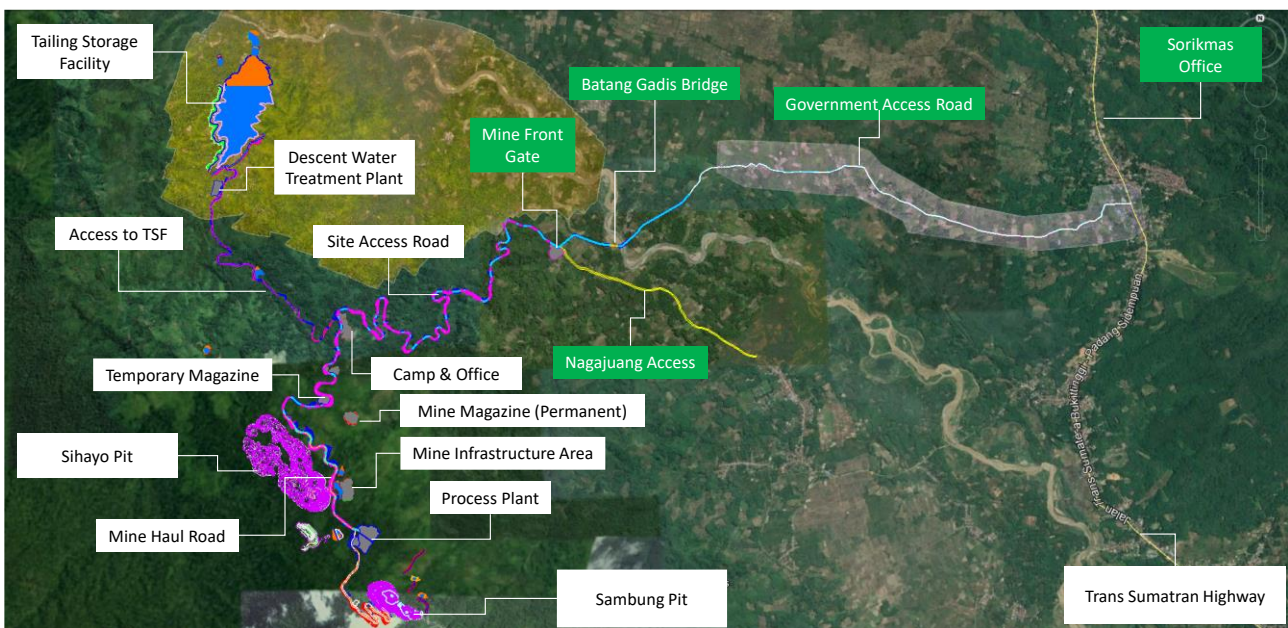
Figure 10. Sihayo Starter Project Site Layout and Site Access
