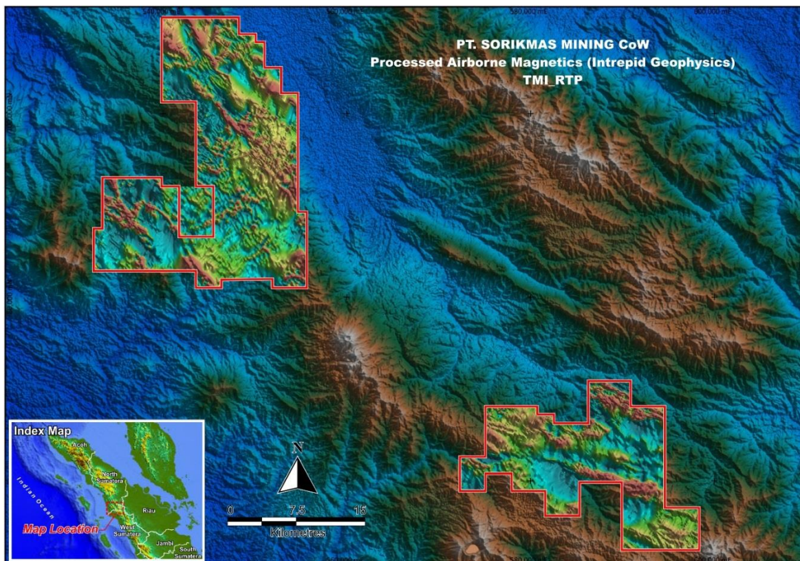
Figure 8. PT Sorikmas Mining CoW – Processed Airborne Magnetics on topography Total Magnetic Intensity / Reduced to Pole
