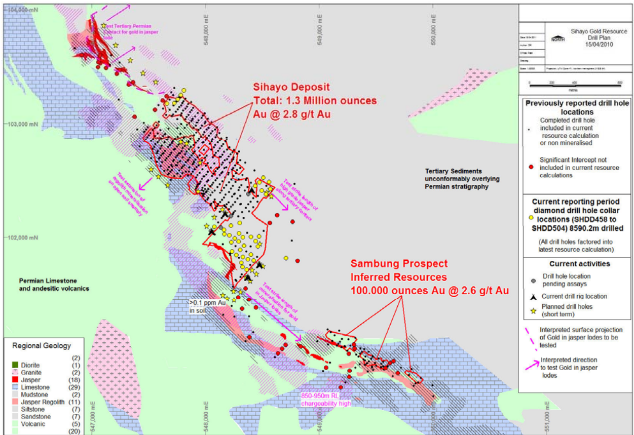
Figure 1: Sihayo and Sambung Resource outline, potential resource extension areas and short term drill hole locations
