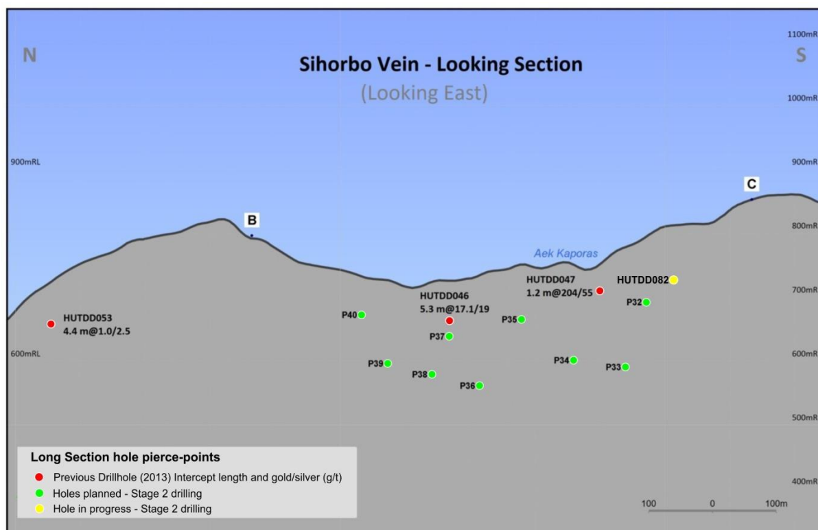
Figure 3: Hutabargot Julu Prospect – Sihorbo Vein Target – Long Section (Looking East)
