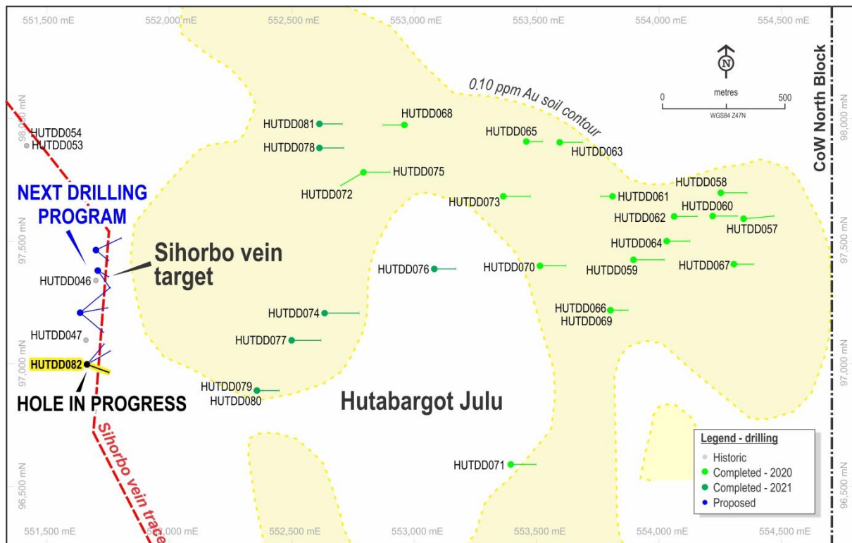
Figure 2: Hutabargot Julu Propsect – Drill Hole Locations & Planned Drill Holes on the Sihorbo Vein Target
